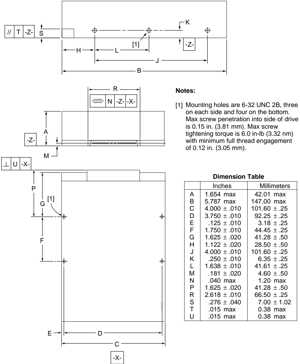
Figure 11. ST136403LC mounting configuration dimensions
