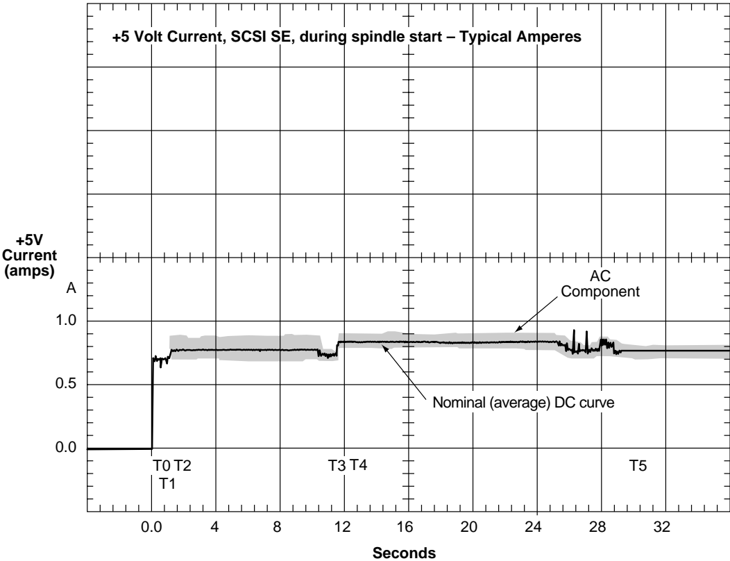
Figure 4. Typical Cheetah 36 SCSI SE mode +5 V current profile
