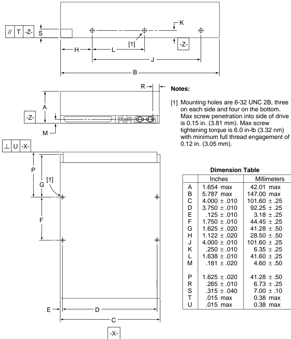
Figure 10. ST136403LW mounting configuration dimensions
