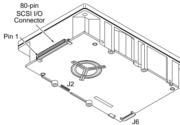
Figure 17. ST136403LC drive physical interface (80-pin J1 SCSI I/O connector)
