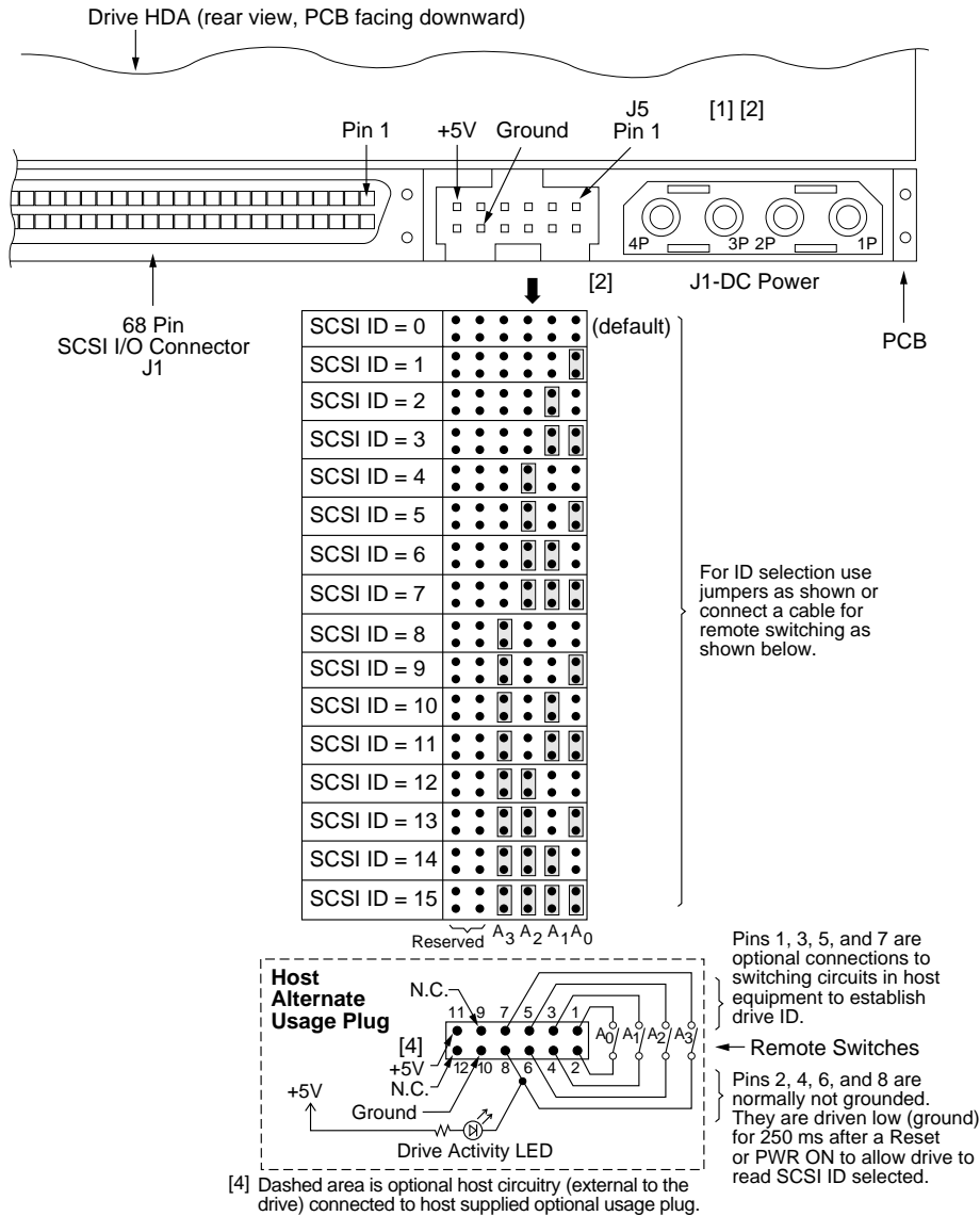
Figure 13. J5 jumper header (on LW models only)
