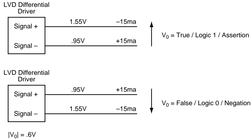
Figure 21. LVD output signals
