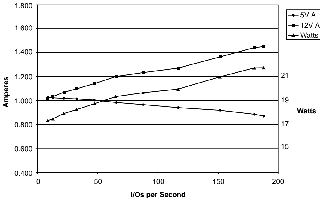
Figure 7. DC current and power vs. input/output operations per second (LVD mode)
