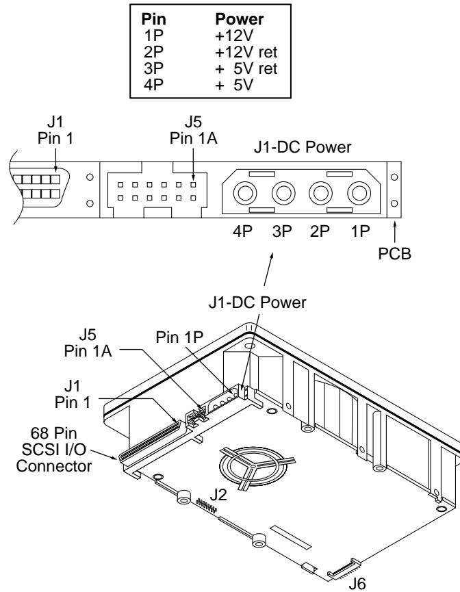
Figure 16. ST136403LW drive physical interface (68-pin J1 SCSI I/O connector)
