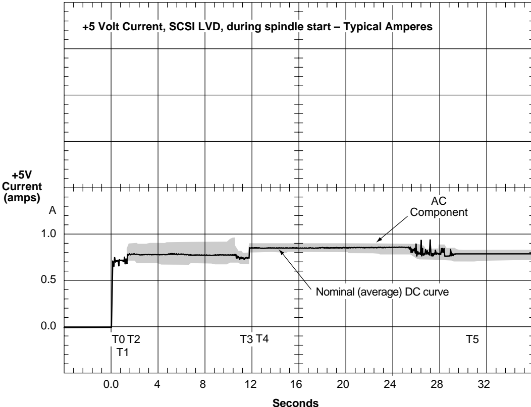
Figure 5. Typical Cheetah 36 SCSI LVD mode +5 V current profile
